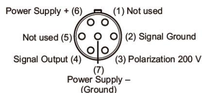
7-pin LEMO plug 1B male (ext. view)
