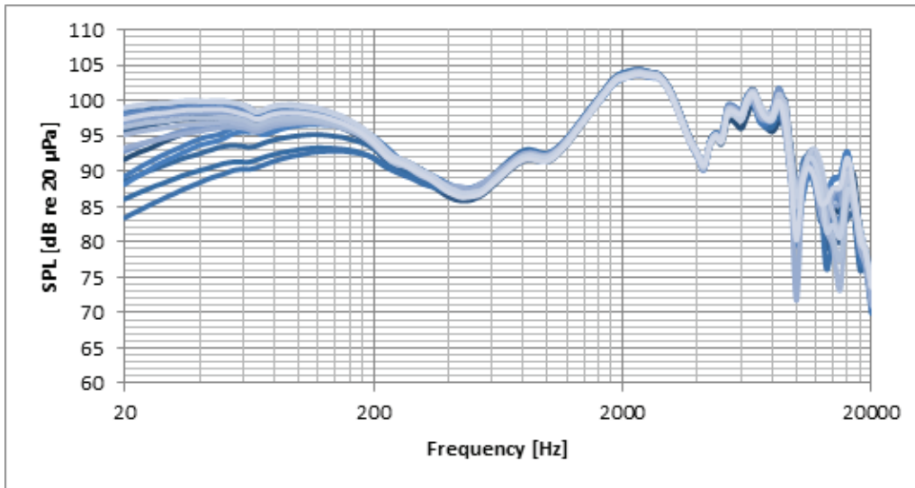
Fig. 17. Twenty measurements with a high quality supra-aural headphone on KEMAR with the standard pinna and ear simulator
