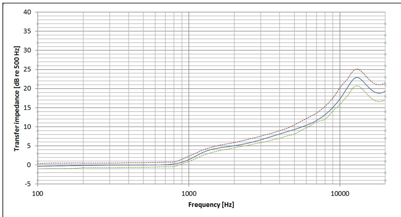
Typical frequency response for RA0401
