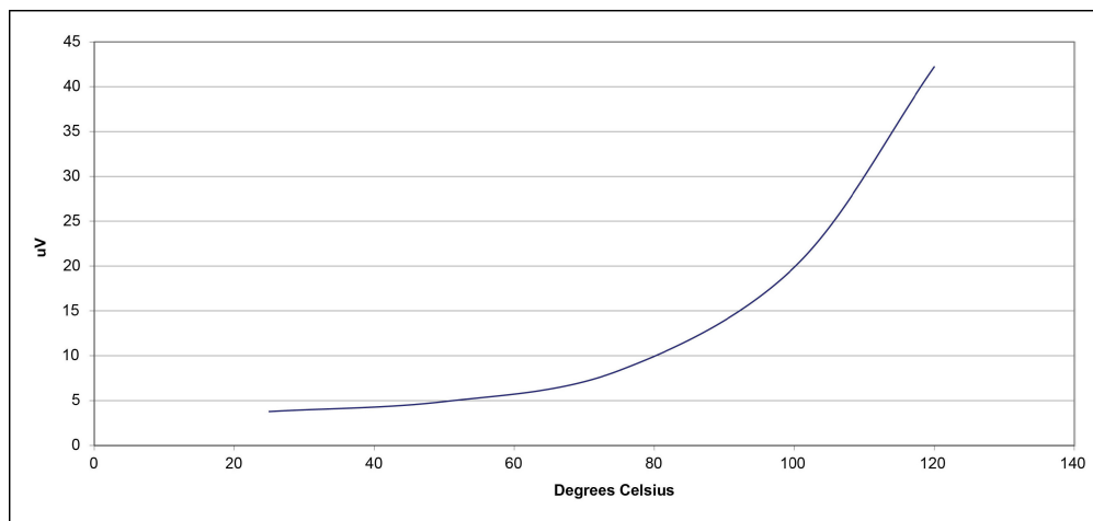
Noise vs. temperature, linear 20 Hz - 20 kHz
