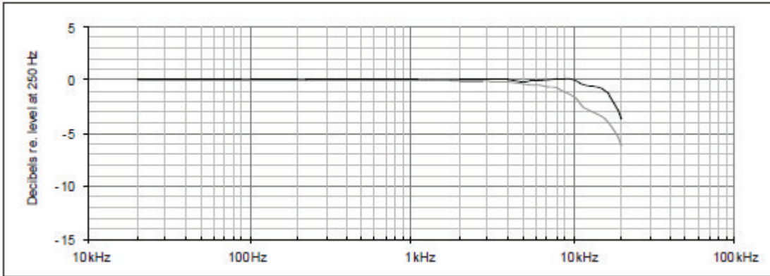
Typical frequency response. Upper curve shows response in a diffuse sound field (random incidence), lower curve shows pressure response.
