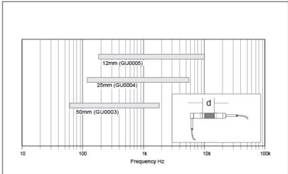
Frequency ranges for different microphone spacers
