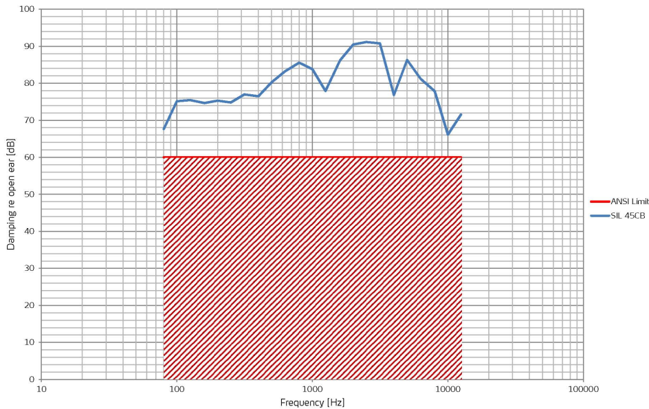
Self Insertion Loss of 45CB, 170 dB
